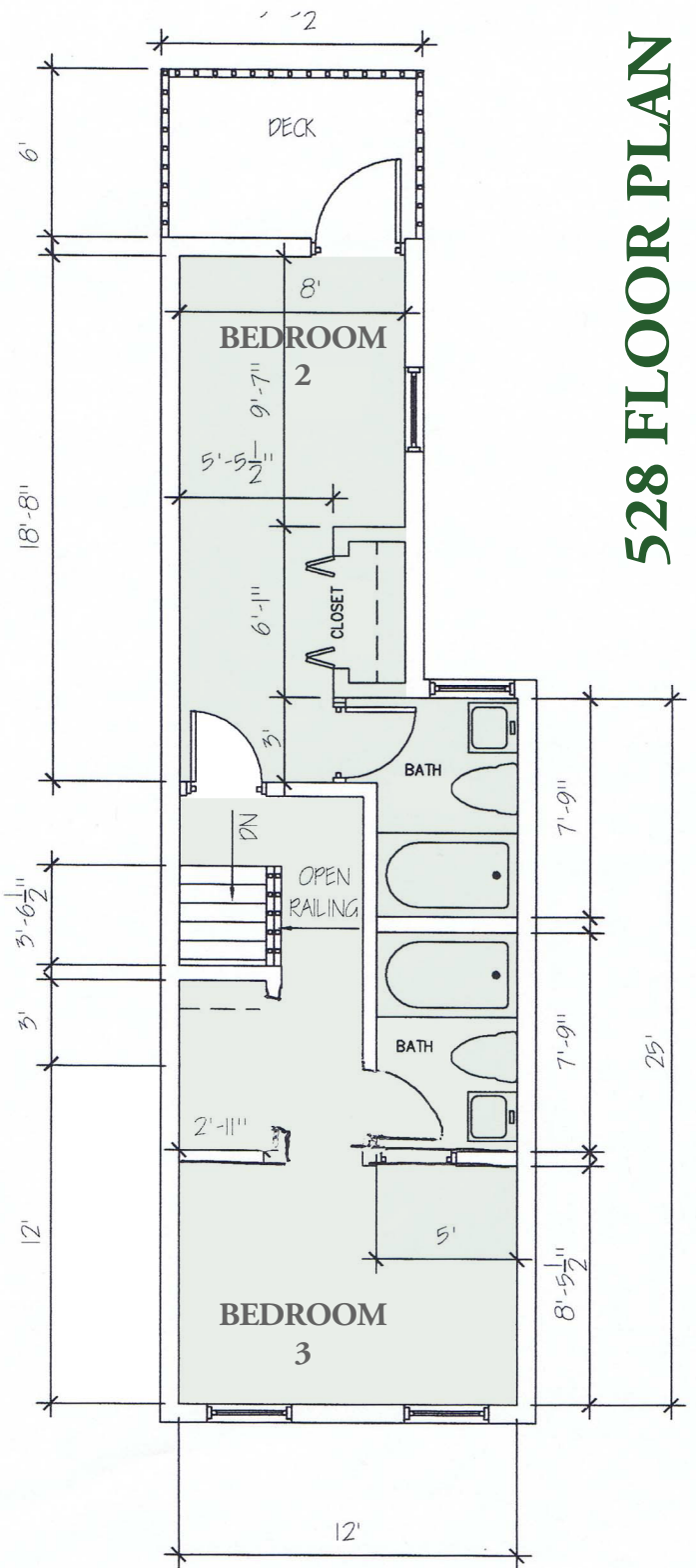
Second Floor - 3/16" 1'- 0"
